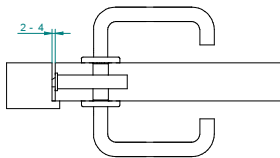
Holgura entre marco y puerta. Gap between frame and door
